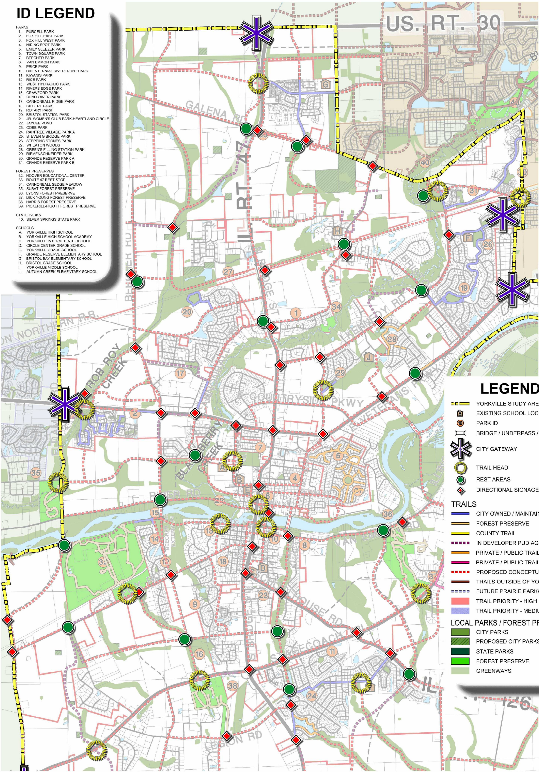
EXHIBIT N - GATEWAYS & WAYFINDING SIGNAGE DETAIL
